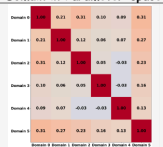
Orthogonality of Selected Domain in Parameter-space
