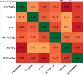
Orthogonality of Selected Domain in Embedding-space
